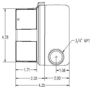
General Dimensions Side and Back Views (All Dimensions in Inches)
